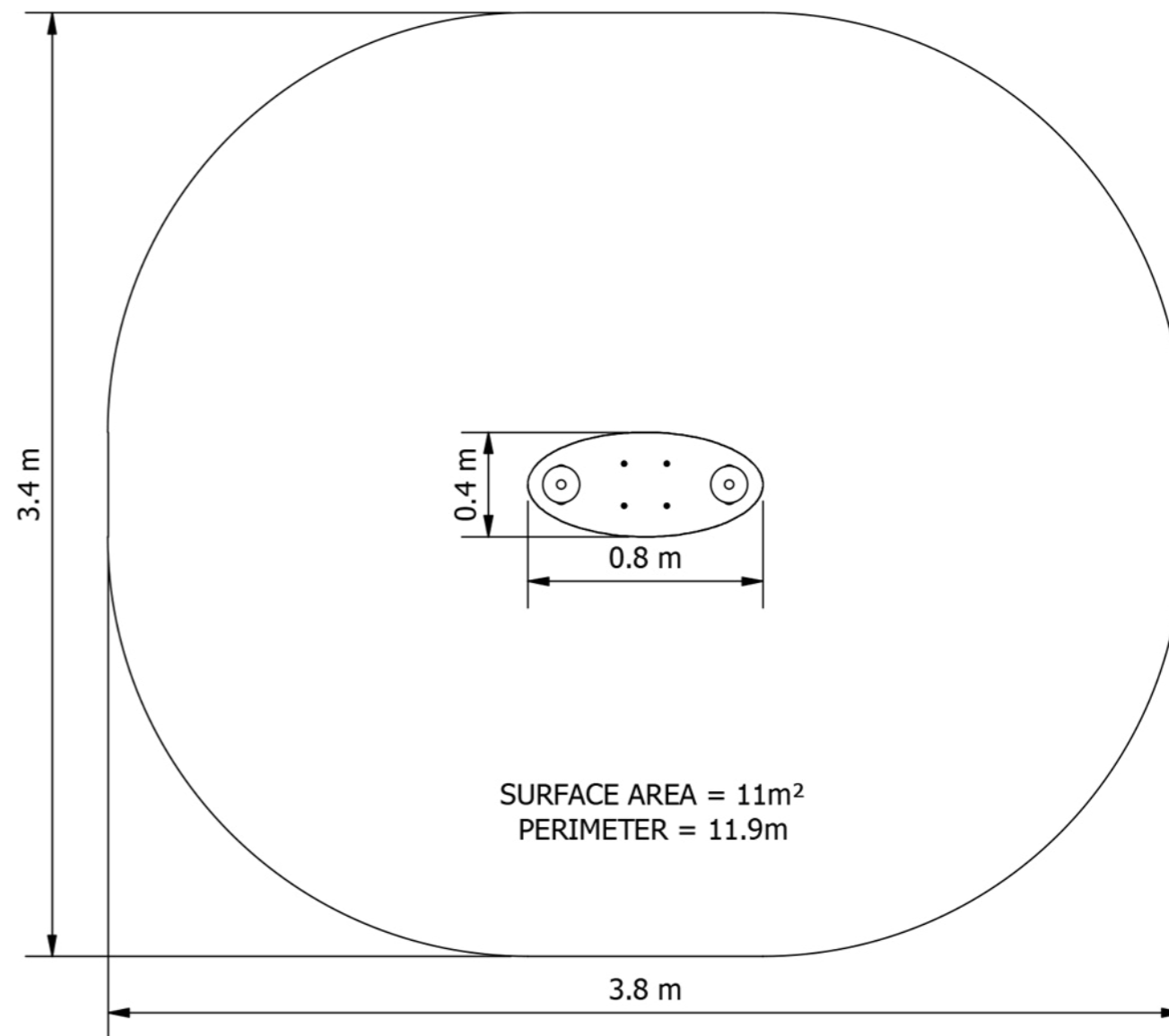
Plan View
