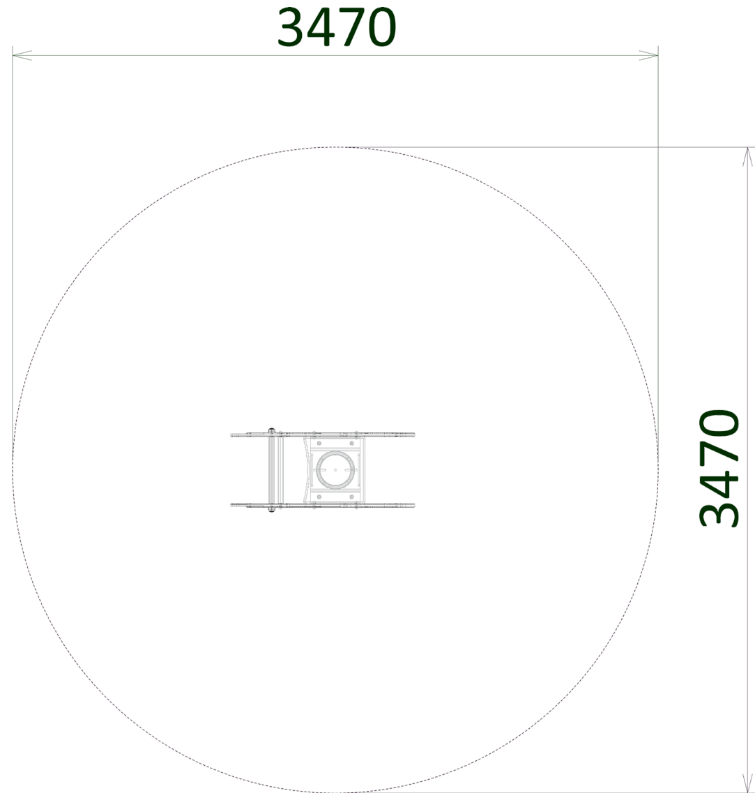
Plan View
